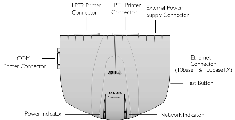
Plan view of the AXIS 5600+
